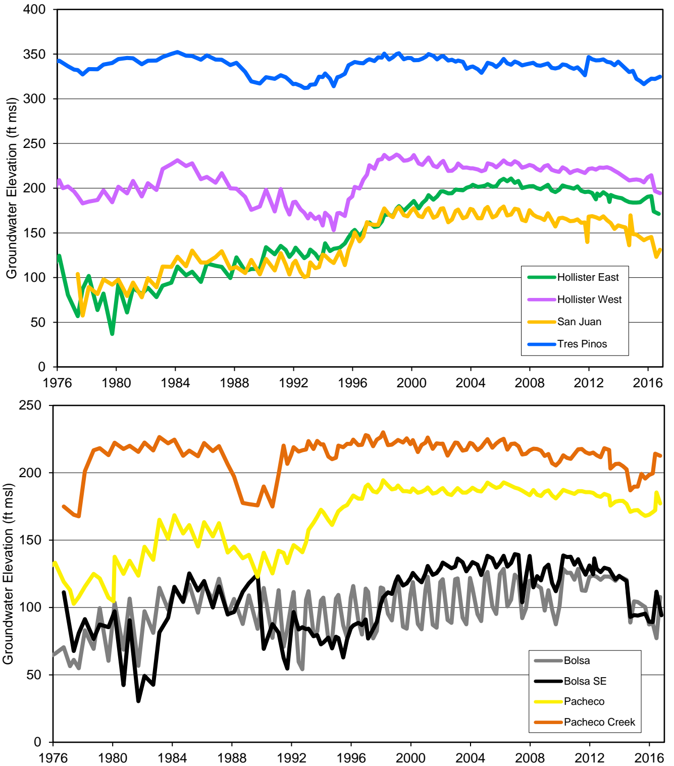
Figure 15. Composite Hydrographs
