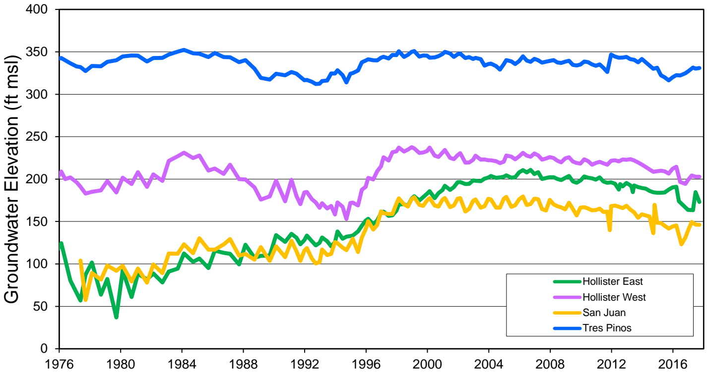
Figure 12. Composite Hydrographs
