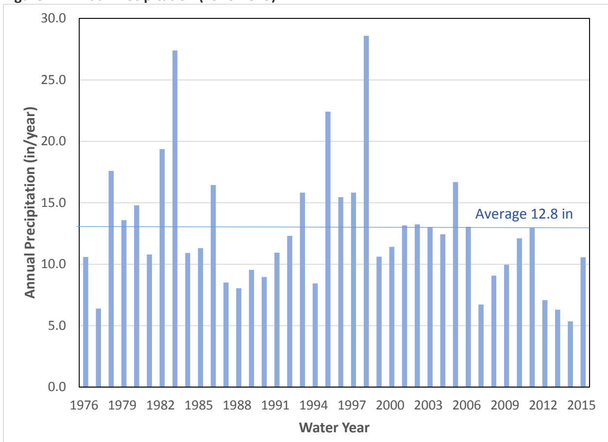
Figure 4. Annual Precipitation (1976-2015)
