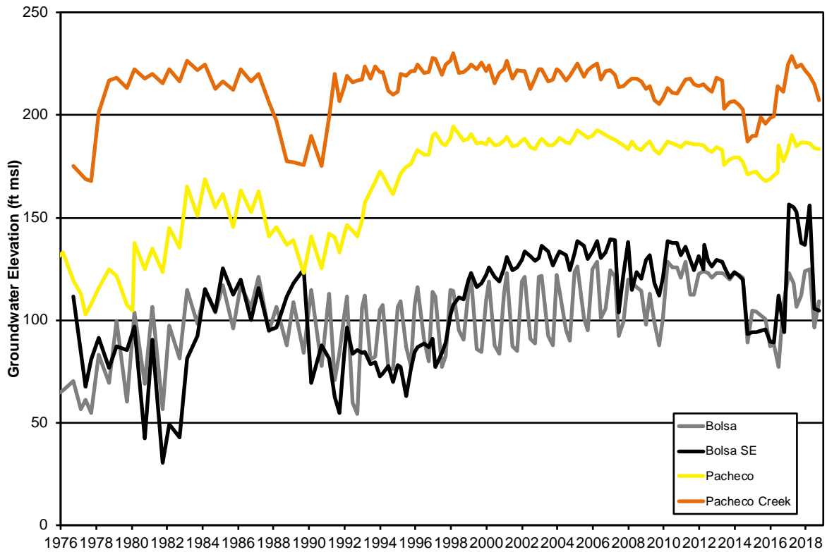
Figure 3-8 Composite Hydrographs
