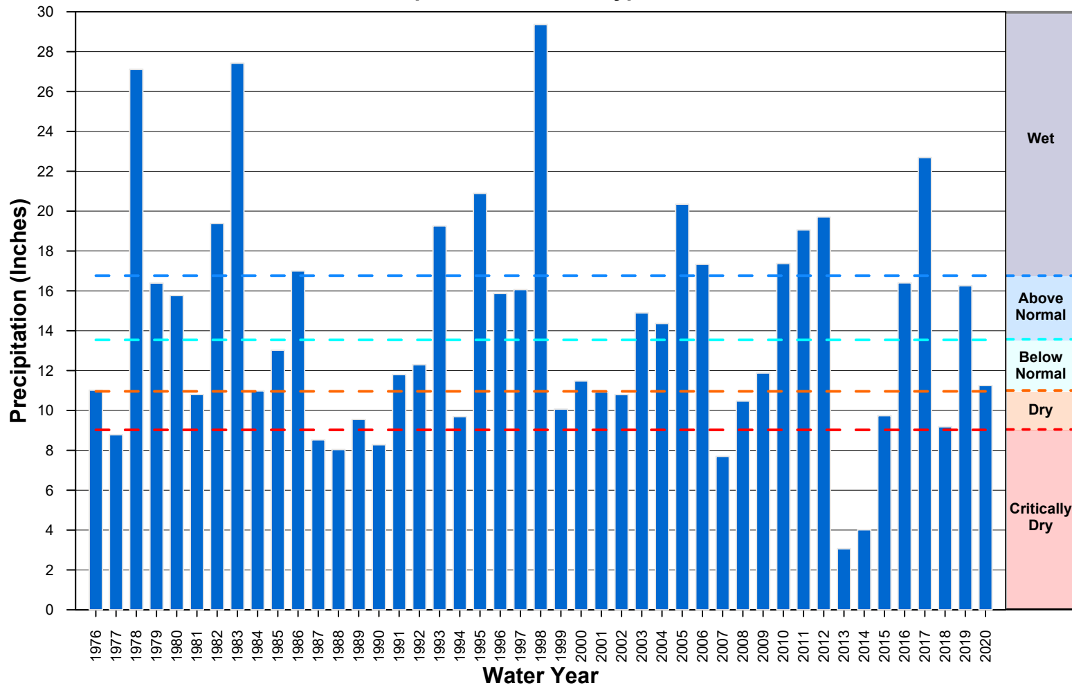
Figure 3-2 Annual Precipitation 1976-2020
