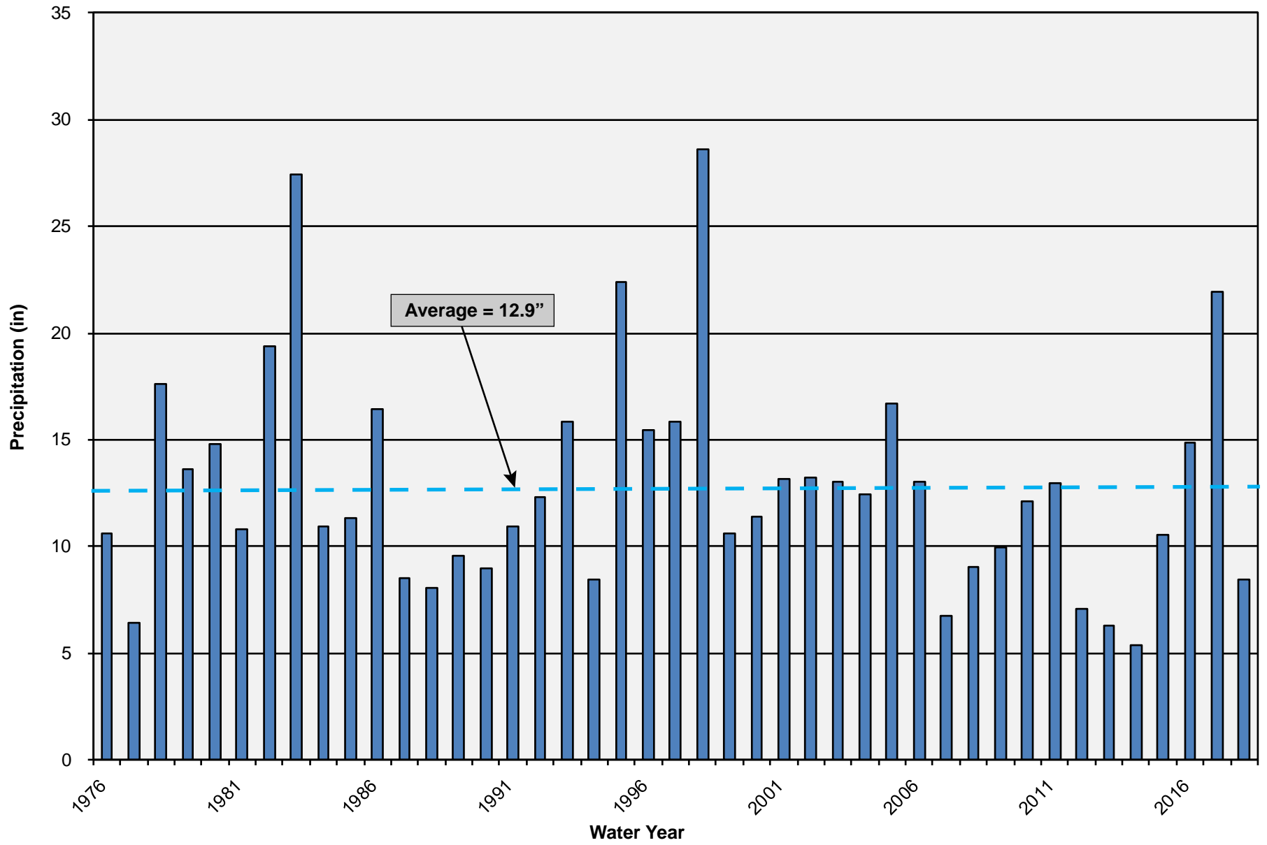
Figure 3-2 Annual Precipitation 1976 - 2018
