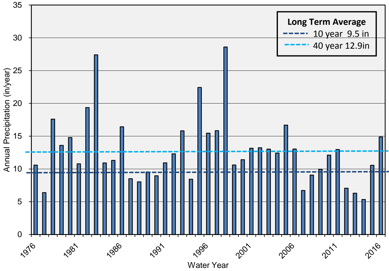
Figure 4. Annual Precipitation (1976-2016)
